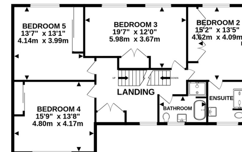
1ST FLOOR 1438 sq.ft. (133.6 sq.m.) approx.
